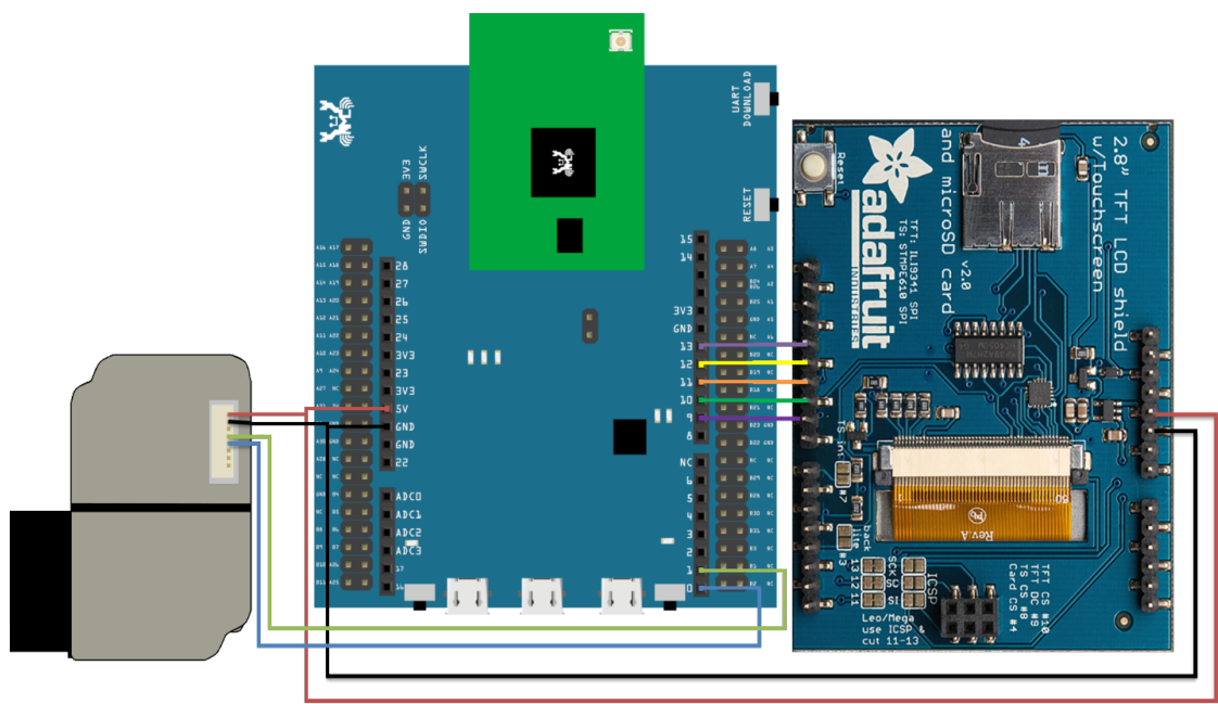
RTL8722DM / RTL8722CSM and Adafruit 2.8” TFT LCD Wiring Diagram:
